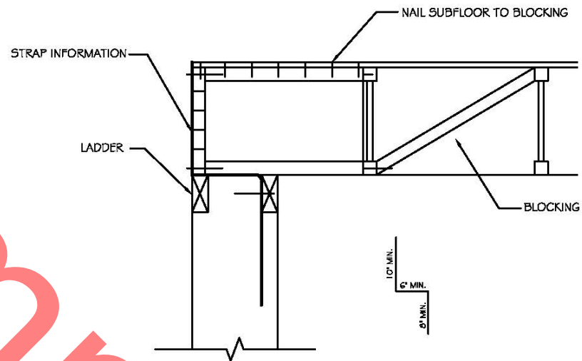
LATERAL BLOCKING DETAIL - JOISTS PARALLEL
